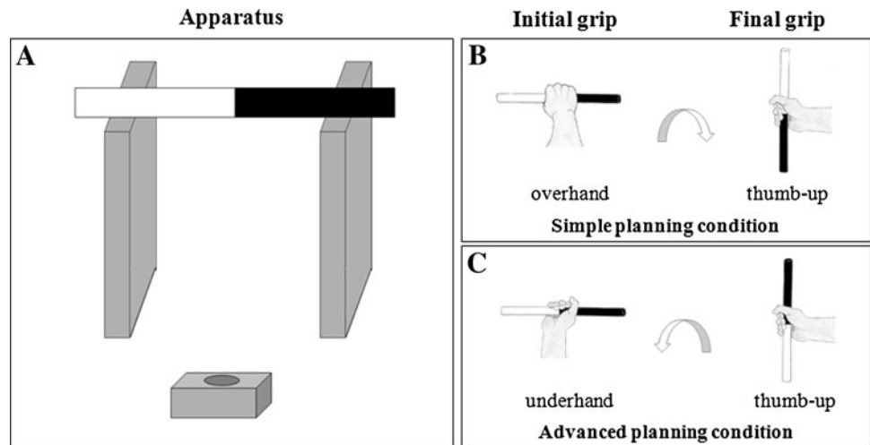
Fig. 1 The apparatus used in the grasping and placing task consisted of a cradle, a wooden bar, and a target. One end of the bar was painted black , and the other end was painted white . a Depicts the bar positioned so that the black end of the bar is facing the right. b and c illustrate representative initial and final grasp postures for the simple and advanced planning condition, respectively. The arrow serves to indicate the direction in which the bar is to be rotated
