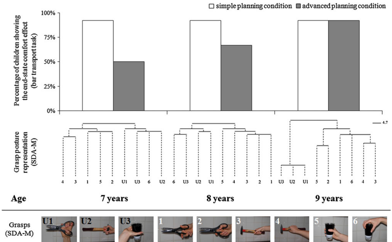
Fig. 2 Top panel: end-state comfort satisfaction (proportion of children) in the bar transport task for the simple (white bars) and advanced planning condition (grey bars). Middle panel: the representational structures for comfortable and uncomfortable grips for the 7-year old children, the 8-year old children and the 9-year old children. Depicted
