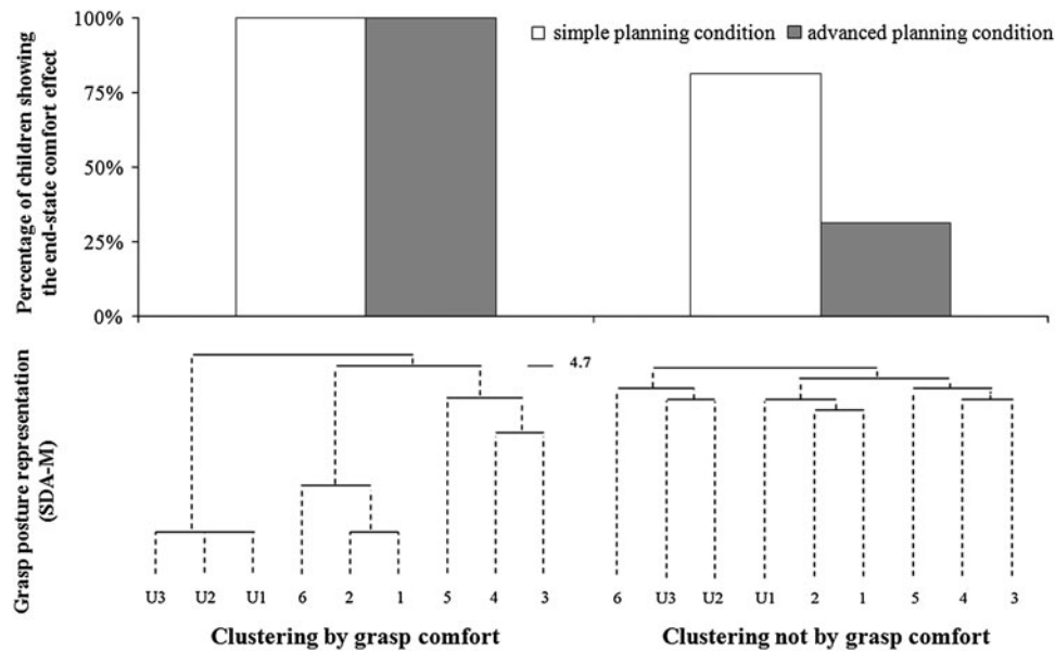
Fig. 3 Results of the bar transport task when participants were grouped according to their clustering in the SDA-M task. Top panel: percentage of children who satisfied end-state comfort in the bar transport task for the simple ( white bars ) and advanced planning condition ( grey bars ). Bottom panel: mental representation of grasp postures
